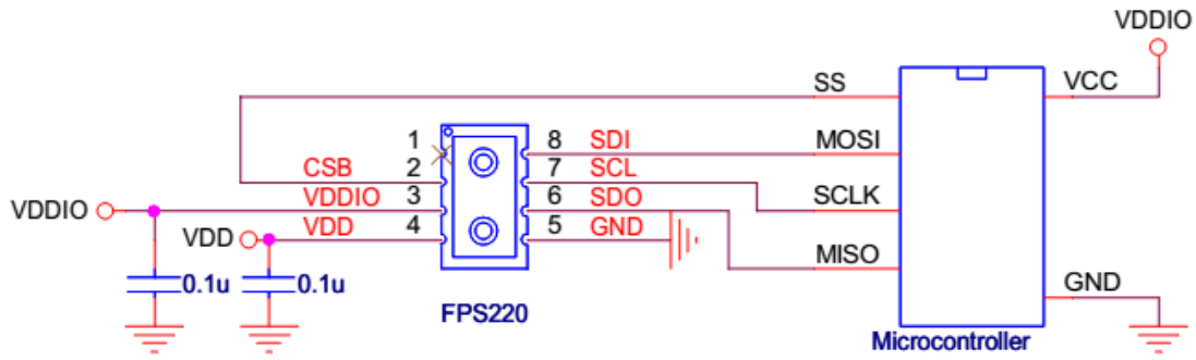
Figure 4.2 Application circuit for SPI interface
